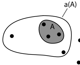
Figure 7: Pseudoclosure of A
