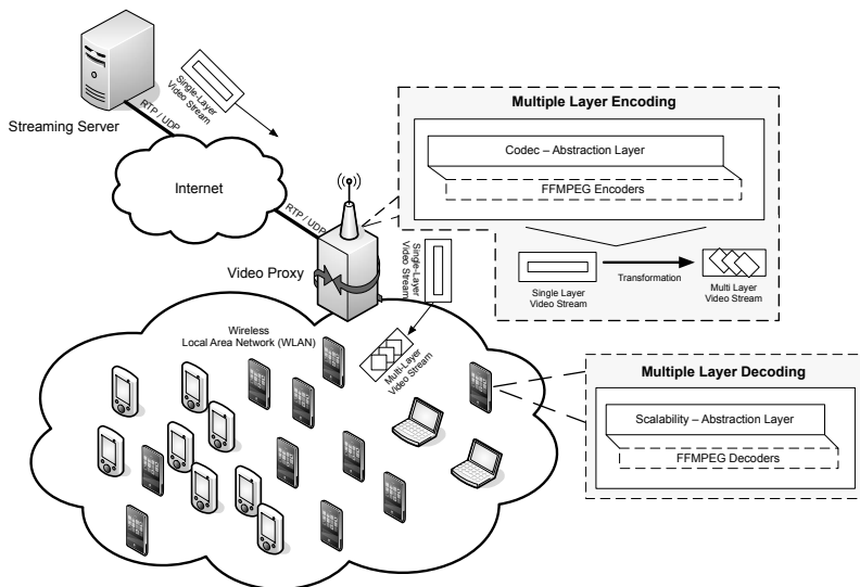
Figure 4: Scalable Video Coding at the Application Layer
