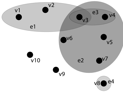
Figure 5: Hypergraph
