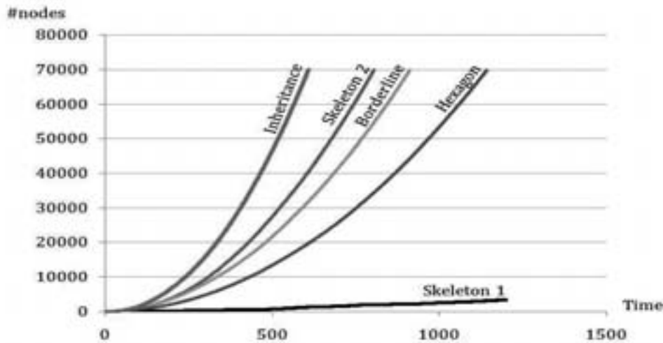
Figure 7: Nodes included in the structure over time
