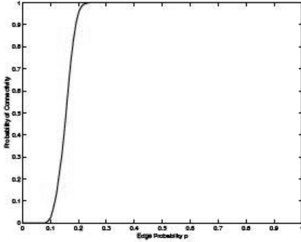
Figure 2: Phase transition in the probability of connectivity in the Bernoulli model (with n=15 ). Source: [KWB01].
