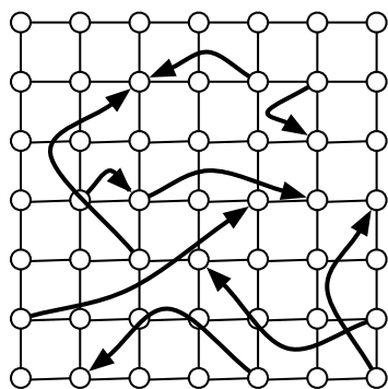
Figure 3: Kleinberg Small-world
