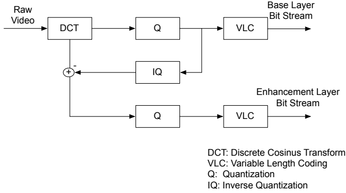
Figure 10: Block diagram Scalable Fidelity Decoder
